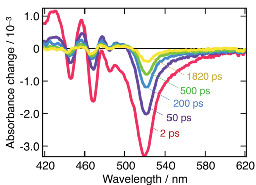
Fig. 2 Transient absorbance spectra of a suspension of \text{CH}_3\text{NH}_3\text{PbBr}_3 nanoparticles in chlorobenzene at different time delays following \lambda_{\text{ex}} = 390 nm pulsed excitation. Red: t = 2 ps, purple: t = 50 ps, blue: t = 200 ps, green: t = 500 ps, and yellow: t = 1820 ps.
