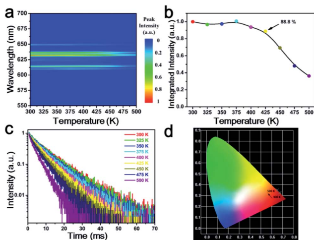
Fig. 4 (a) Temperature-dependent emission spectra of K_2LiGaF_6:Mn^{4+} from 300 K to 500 K, (b) PL integrated intensity, (c) decay time and (d) CIE chromaticity coordinates of K_2LiGaF_6:Mn^{4+} from 300 K to 500 K.
