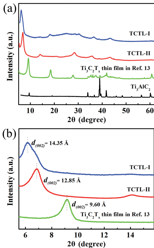
Fig. 2 (a) XRD patterns of the TCTL-I, TCTL-II, the previous Ti 3 C 2 T x thin film in ref. 13, and Ti 3 AlC 2 powder and (b) the corresponding enlarged XRD patterns.
