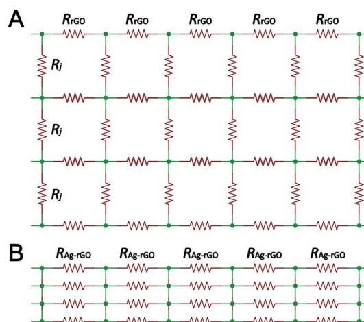
Fig. 6 Illustration of the resistor network model describing a four-layer stacked (A) rGO film and (B) Ag-rGO film. For rGO film, large resistance of individual rGO sheets and rGO-rGO junctions ( R_j ) result in a large sheet resistance. For Ag-rGO films, the resistance of rGO sheets decreases due to the n-doping effect, and AgNPs bridge the resistive rGO-rGO junctions. R_{rGO} and R_{Ag-rGO} ( < R_{rGO} ) denote the intrinsic resistance of individual rGO sheets and Ag-rGO hybrid sheets, respectively.
