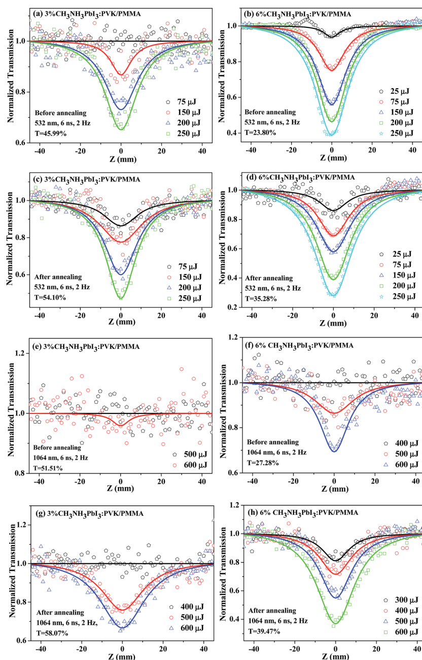
Fig. 3 Typical open-aperture Z-scan data of the \text{CH}_3\text{NH}_3\text{PbI}_3:\text{PVK}/\text{PMMA} films with different \text{CH}_3\text{NH}_3\text{PbI}_3:\text{PVK} concentrations. The annealing condition: 200 ^\circ\text{C} for 30 min in \text{N}_2 .
