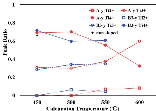
Fig. 3 The peak ratios of \text{Ti}^{2+}(\beta_1) , \text{Ti}^{3+}(\beta_2) and \text{Ti}^{4+}(\beta_3) for the samples synthesized by method A (A-γ, red) and B (B3-γ, blue) as a function of calcination temperature (γ). The ratio of \text{Ti}^{4+}(\beta_3) for non-doped sample is indicated by a cross.
