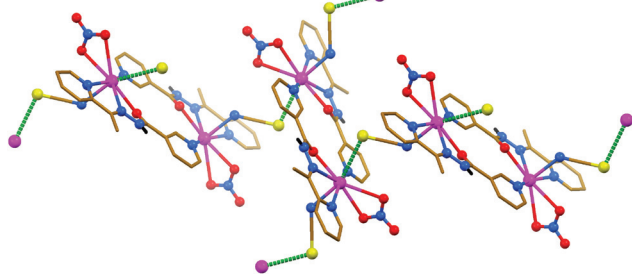
Fig. 6 Crystal structure of [\text{Pb}_2(\text{HL})_2(\text{NO}_3)_2(\text{NCS})_2] (CH hydrogen atoms are omitted for clarity). Tetrel bonds \text{Pb}\cdots\text{S} are shown as dashed lines. Color code: C = gold, H = black, N = blue, O = red, Pb = magenta, S = yellow.
