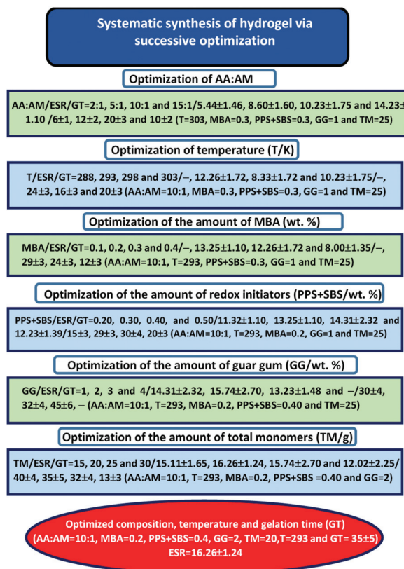
Scheme 2 Systematic optimization.
