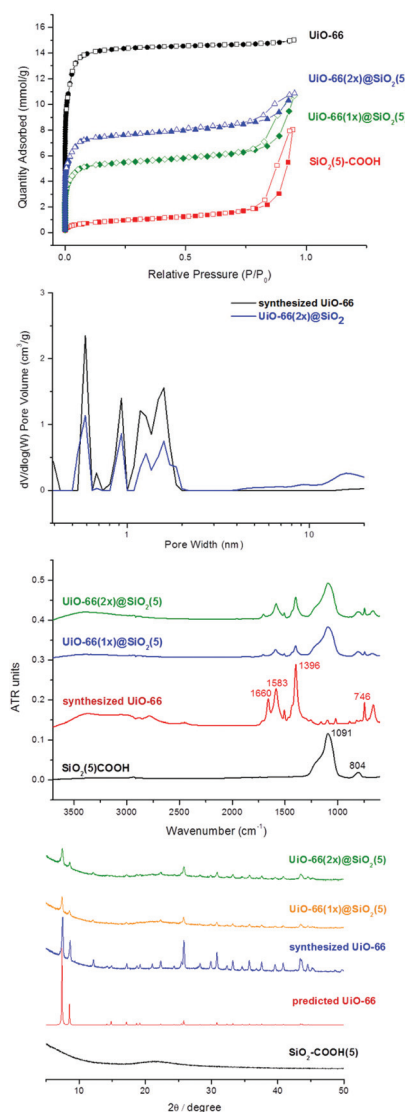
Fig. 2 (a) \text{N}_2 adsorption (filled) and desorption (open) isotherms at 77 K for \text{SiO}_2(5)\text{-COOH} (red squares), synthesized UiO-66 (black circles), UiO-66(1 \times )@ \text{SiO}_2(5) (green diamonds) and UiO-66(2 \times )@ \text{SiO}_2(5) (blue triangles) core-shell particles. (b) Pore size distribution curves obtained using the density functional theory (DFT) model for synthesized UiO-66 (black) and UiO-66(2 \times )@ \text{SiO}_2(5) (blue) core-shell particles. (c) FT-IR spectra of \text{SiO}_2(5)\text{-COOH} (black), synthesized UiO-66 (red), UiO-66(1 \times )@ \text{SiO}_2(5) (blue) and UiO-66(2 \times )@ \text{SiO}_2(5) (green) core-shell particles. (d) PXRD patterns of \text{SiO}_2\text{-COOH}(5) (black), predicted UiO-66 (red), synthesized UiO-66 (blue), UiO-66(1 \times )@ \text{SiO}_2(5) (orange) and UiO-66(2 \times )@ \text{SiO}_2(5) core-shell particles (green).
