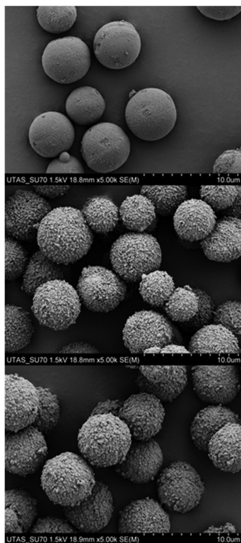
Fig. 1 Scanning electron microscopy images of \text{SiO}_2(5)\text{-COOH} (top), UiO-66(1 \times )@ \text{SiO}_2(5) (middle) and UiO-66(2 \times )@ \text{SiO}_2(5) (bottom) particles.
