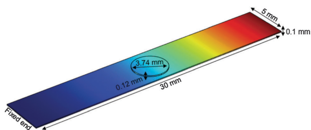
Fig. 7 Finite element calculation of freely vibrating nanostructured scaffold with retina on top (circle). One end of the scaffold is fixed, while the other end vibrates freely. The color code shows the vibration amplitude from no extension (blue) to the maximum (red).
