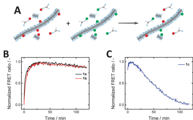
Fig. 5 (A) Schematic of FRET exchange experiment. (B) FRET experiments of 1a and 1b show similar exchange kinetics, while (C) 1c shows erratic behaviour due to poor self-assembly ( c_{\text{BTA}} = 1 \times 10^{-5} M).
