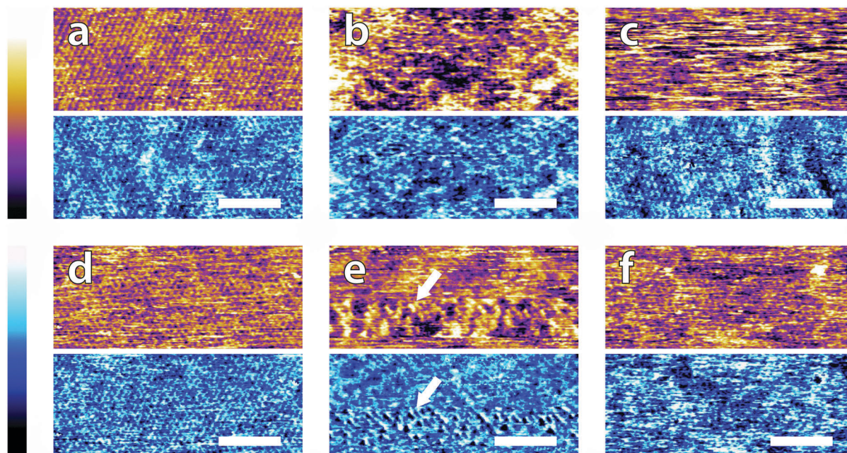
Fig. 3 High magnification AFM images of mica topography (upper) and phase (lower) in buffer solutions. In MES (a) the hexagonal symmetry of the lattice can be clearly resolved despite infrequent horizontal defects. Regular epitaxial modulations are visible in the phase. In HEPES (b) the symmetry is again clear, but modulated by large height variations in both topography and phase. In Monosodium phosphate (c) the topography image displays no atomic features but they can be occasionally resolved in the corresponding phase image. In SSC (d) the mica lattice is perceptible with larger features similarly to in (a). In Tris (e), large features consistent with those in Fig. 2e are visible in the upper part of the image. Occasionally, the tip jumps (arrow) revealing a structured mesh. In ultrapure water (f) atomic-level features are visible alongside point-like deformities. The scale bar is 5 nm. Colour scales: the height is 150 pm and phase is 10^\circ .
