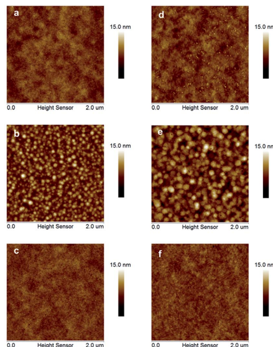
Fig. 6 AFM morphology images (2 \mu\text{m} \times 2 \mu\text{m} ). (a) PDTPPO-IDT pure film, RMS: 0.88 nm. (b) PDTPPO-IDT : PC 71 BM blend film without DIO, RMS: 1.62 nm. (c) PDTPPO-IDT : PC 71 BM blend film with 3% DIO, RMS: 0.68 nm. (d) PDTPPO-IDTT pure film, RMS: 0.99 nm. (e) PDTPPO-IDTT : PC 71 BM blend film without DIO, RMS: 1.87 nm. (f) PDTPPO-IDTT : PC 71 BM blend film with 3% DIO, RMS: 0.72 nm.
