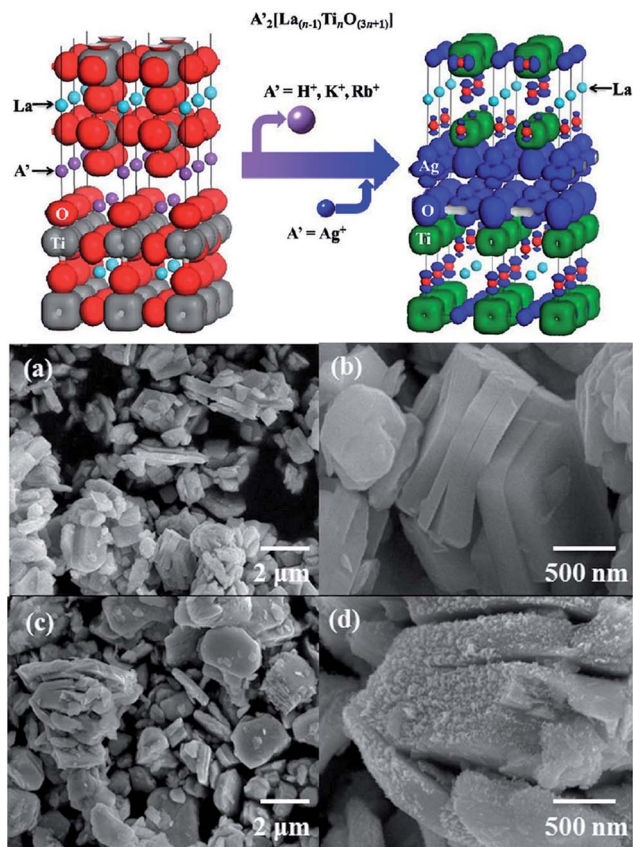
Fig. 8 (Top) Electron density plot of A'_2[La_{(n-1)}Ti_nO_{(3n+1)}] and Ag_2^-La_2Ti_3O_{10} . (a and b) FESEM images of solid-state prepared Rb_2La_2Ti_3O_{10} . (c and d) Silver-exchanged Ag_2La_2Ti_3O_{10} in AgNO_3 flux (ref. 30 Copyright 2013, American Chemical Society).
