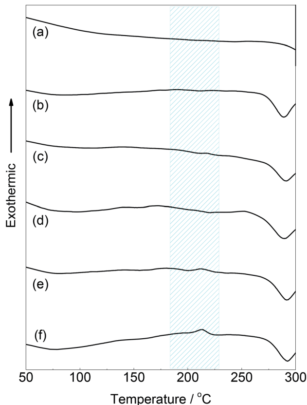
Fig. 5 DSC traces of (a) the native silk fibroin and PPE-modified silks with different feed concentrations of DMP (b: 0.02 M, c: 0.04 M, d: 0.06 M, e: 0.08 M, and f: 0.10 M) in the first heating scan at 20\text{ }^{\circ}\text{C min}^{-1} .
