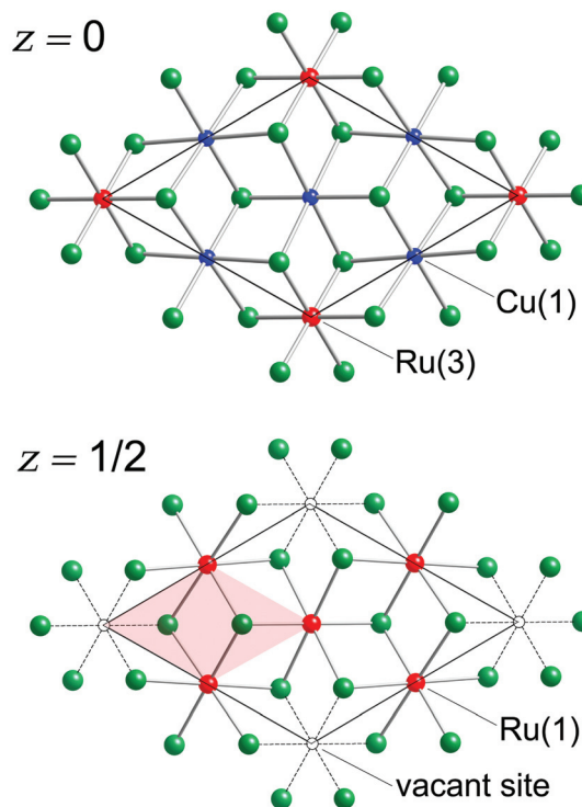
Fig. 2 The hcp sub-lattice of Sb atoms in the \text{Cu}_3\text{Ru}_6\text{Sb}_8 structure, shown as cut-outs at two different z -levels. Both projections are down the [001] direction. The Cu(1), Ru(1), and Ru(3) atoms forming slabs of fused octahedra are depicted. The vacant octahedral sites ( 1/8 of all, shown as open circles) and the would-be NiAs sub-cell (shaded area) are also emphasized.
