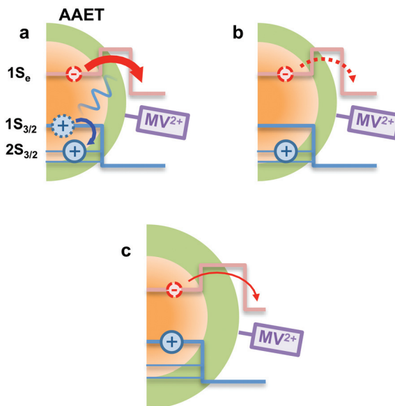
Fig. 8 Schematic illustration of the AAET process. (a): In the AAET process, electron transfer to \text{MV}^{2+} is accompanied by the excitation of the 1S_{3/2} hole to higher levels. (b): The Auger process lacks the 1S_{3/2} to 2S_{3/2} hole transition, leading to inefficient AAET. (c): With thick shell, the Auger-assisted channel is cut off due to the weak electron–hole coupling.
