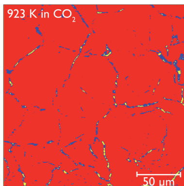
Fig. 12 Reconstructed tomography slices of CaO after reacting under CO 2 for 50 minutes. The colours show the phase segregation of the image into pores (yellow), CaCO 3 (dark blue) and CaO (red).
