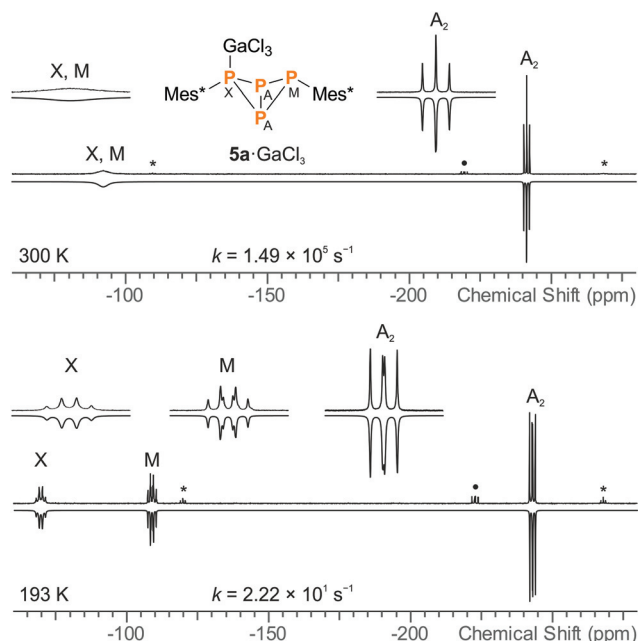
Fig. 4 Experimental (up) and simulated (down) ^{31}\text{P} NMR spectra of 5a -GaCl 3 at 27 °C (top) and -80 °C (bottom), demonstrating the dynamic exchange of the GaCl 3 moiety in solution (* = 5a , • = impurity of 5b -GaCl 3 ). GaCl 3 was added to 5a in slightly sub-stoichiometric amounts (0.95 eq.) so the non-coordinating bicyclic phosphane was detectable in the NMR spectrum.
