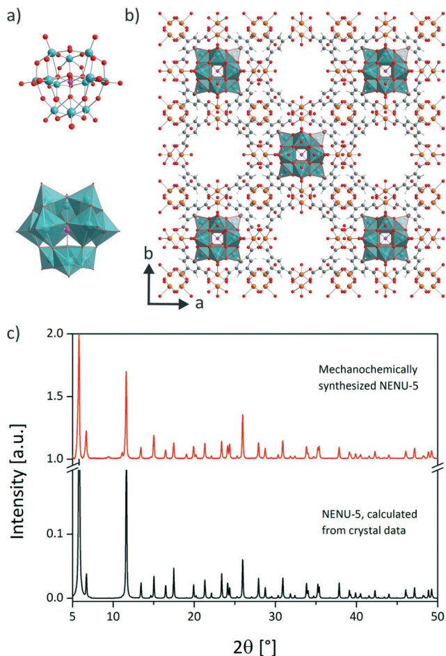
Fig. 1 a) Structure of the Keggin-type POM [P 12 O 40 ] 6- shown as ball-and-stick and polyhedra model. b) Structure of NENU-5 consisting of empty pores and pores filled with Keggin ions (polyhedra). Orange: copper, turquoise: molybdenum, pink: phosphorus, red: oxygen, grey: carbon, light grey: hydrogen. c) Comparison of the diffraction pattern of the mechanochemically synthesised NENU-5 with the calculated diffraction pattern.
