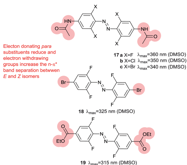
Fig. 9 Tetra- ortho halogen substituents separate the n\text{-}\pi^* transition energies of E and Z isomers, impart resistance to glutathione reduction and lead to long lived Z -isomers.
