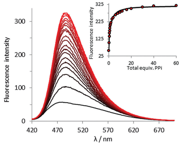
Fig. 4 Fluorescence emission spectra of 1-Zn 2 (5 \mu\text{M} ) in response to PPI (0–300 \mu\text{M} ) in HEPES (5 mM, 145 mM NaCl, pH 7.4) at 25 °C. \lambda_{\text{ex}} = 390 nm, slits = 5 nm/5 nm. Inset: Binding isotherm (–) obtained by fitting the observed fluorescence intensities at 480 nm (●) to a 1:1 binding model using non-linear regression.
