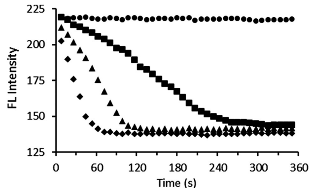
Fig. 5 Real-time assay of PPI (80 \mu\text{M} ) hydrolysis catalysed by different amounts of pyrophosphatase (● = 0 units, ■ = 0.5 units, ▲ = 1.0 units, ◆ = 2.0 units) in the presence of 3-Zn 2 (15 \mu\text{M} ) in Tris buffer (10 mM, 10 mM MgCl 2 , pH 7.5) at 30 °C, \lambda_{\text{ex}} = 390 nm, slits = 5 nm & 5 nm.
