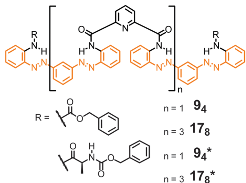
Fig. 8 Photoswitchable oligoamide foldamers composed of azobenzene and pyridine moieties terminated with achiral units ( 9a and 17a ) and chiral units ( 9a* and 17a* ), the latter to facilitate analysis by CD spectroscopy. 43,92 Throughout, oligomers are named by giving the number of aromatic repeat units (here: 9 or 17) followed by the number of incorporated azo (N=N) bonds in subscripts (here: 4 or 8).
