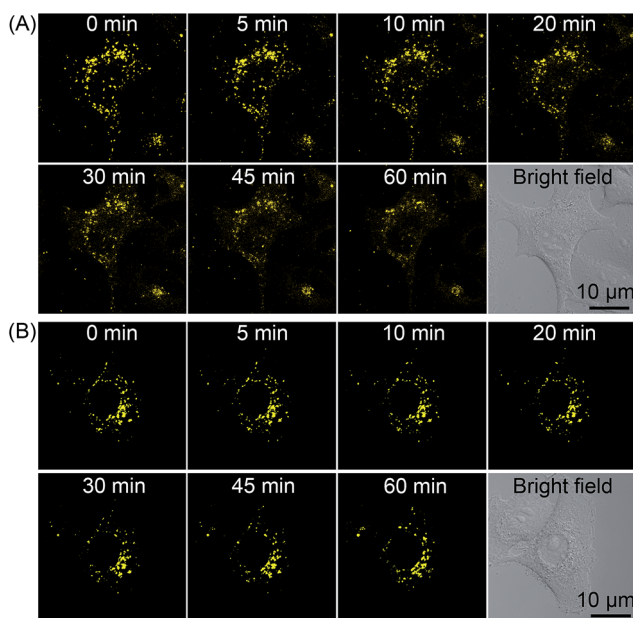
Fig. 10 Real-time monitoring of lysosomal integrity in A549 cells loaded with 2 (10 \mu\text{M} , 12 h) (A) with or (B) without PDT treatment (120 s, 4.8 J \text{cm}^{-2} ).
