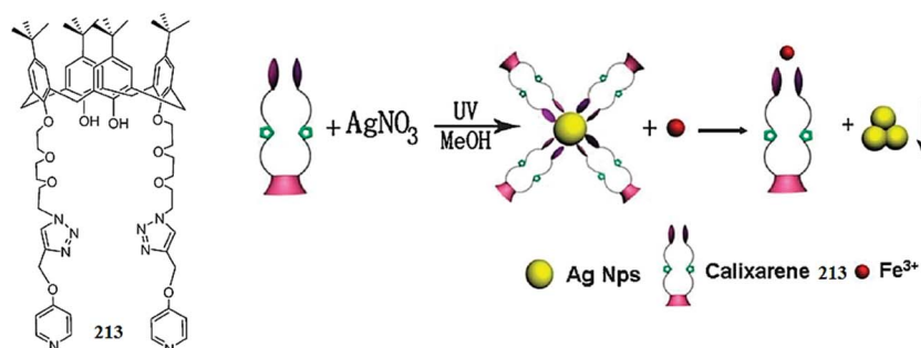
Fig. 178 Chemical structure of calix[4]arene 213 , synthesis of 213 –Ag NPs and schematic of Fe 3+ -induced 213 –Ag NP aggregation.
