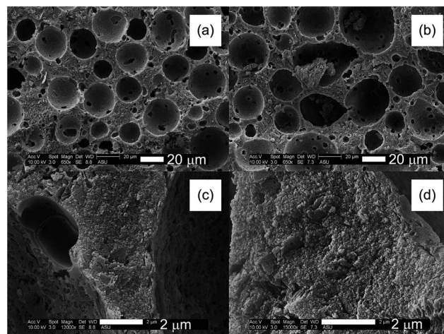
Fig. 4 SEM images of GEO in (a) and (c) (scale bar = 20 and 2 \mu m , respectively) and of CaGEO-4 in (b) and (d) (scale bar = 20 and 2 \mu m , respectively).
