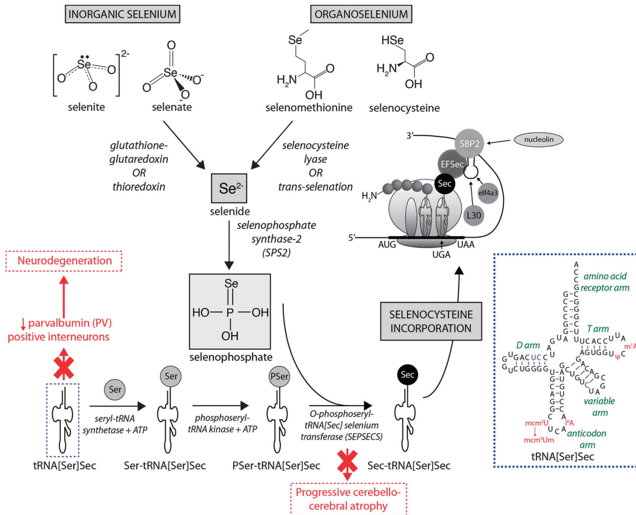
Fig. 1 Selenoprotein synthesis pathway. Dietary Se intake, as either inorganic or organic species is metabolised to Se 2- , and the SeH 3 PO 3 , which is incorporated into proteins via a unique tRNA pathway, where a seryl (Ser) residue is replaced with selenocysteine (Sec) prior to integration into mammalian proteins. Deficiencies in key metabolic factors involved in selenoprotein synthesis have been associated with specific neurological disorders, marked here in red. The inset in the dashed blue box is the simplified cloverleaf structure of mammalian tRNA[Ser]Sec (adapted from Birringer et al. 196 ), showing variable (in blue) and modifiable (in red) bases. Abbreviations: Ψ = pseudouridine; EFSec = Sec elongation factor; eIF4a3 = eukaryotic initiation factor; i 6 A = N 6 -isopentenyladenosine; L30 = ribosomal protein L30; mcm 5 U = 5-methoxycarbonylmethyluridine; m 1 A = 1-methyladenosine; mcm 5 Um = 5-methoxycarbonylmethyluridine-2'-O-methylribose; SBP2 = Sec insertion sequence (SCIS) binding protein-2.
