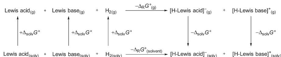
Fig. 2 Born-Haber-Fajans cycle to access the \Delta_r G^\circ_{(g)} and \Delta_r G^\circ_{(solv)} of 1 and B(C 6 F 5 ) 3 in various solvents.
