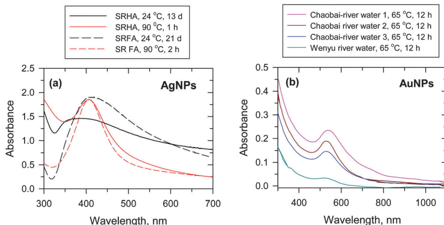
Fig. 5 (a) UV-vis absorption spectra of Ag nanoparticles (AgNPs) in Suwannee river humic acid (SRHA) and Suwannee river fulvic acid (SRFA) at 24 °C and 90 °C at pH 8.0 ( [\text{Ag}^+] = 1 \times 10^{-4} mol \text{L}^{-1} , [\text{SRFA}] = [\text{SRHA}] = 100 mg \text{L}^{-1} ). (Adapted with permission from ref. 12, copyright American Chemical Society). (b) UV-vis absorption spectra of Au nanoparticles (AuNPs) in river water at 65 °C at pH 8.0 ( [\text{Au}^+] = (62.5-1000) \times 10^{-6} mol \text{L}^{-1} , [\text{HA}] = 5-100 mg DOC \text{L}^{-1} , where DOC – dissolved organic carbon). (Adapted with permission from ref. 30, copyright American Chemical Society).
