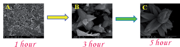
Fig. 9 FESEM images of ZnO nanostructure synthesis after (a) 1 h, (b) 3 h, and (c) 5 h, respectively.
