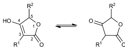
Fig. 1 Tetronic acid tautomers.
