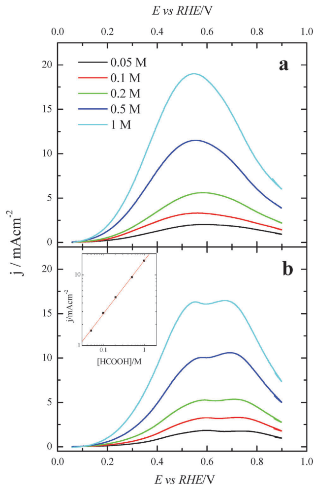
Fig. 9 Positive sweep voltammetric profiles for (a) (100)Pt and (b) (111)Pt nanoparticles with maximum TI coverage in different concentrations of formic acid in 0.5 M H 2 SO 4 . Scan rate: 0.02 V s -1 . Inset: double logarithmic plot of the current density at 0.5 V for the (111)Pt nanoparticles vs. formic acid concentration.
