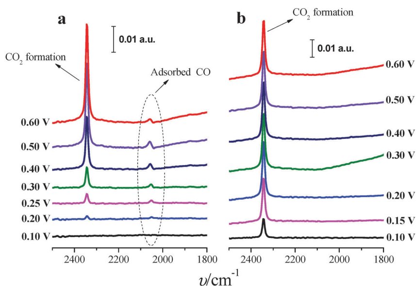
Fig. 8 In situ FTIR spectra for formic acid electro-oxidation on (100)Pt nanoparticles: (a) bare Pt and (b) maximum TI coverage. Reference spectra were taken at 0.05 V. Test solution: 0.05 M formic acid in 0.1 M H 2 SO 4 .
