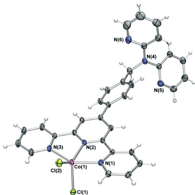
Fig. 1 X-ray structure of [\text{Co}(\text{L})\text{Cl}_2]\cdot 0.25\text{DCM}\cdot 0.5\text{H}_2\text{O} . Solvent molecules have been removed for clarity. Thermal ellipsoids are shown at the 50 percent probability level.
