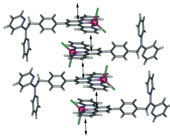
Fig. 2 Representation of the one-dimensional stack that propagates parallel to the crystallographic ab vector in [\text{Co}(\text{L})\text{Cl}_2]\cdot 0.25\text{DCM}\cdot 0.5\text{H}_2\text{O} . Double headed arrows indicate the presence of arene–arene interactions.
