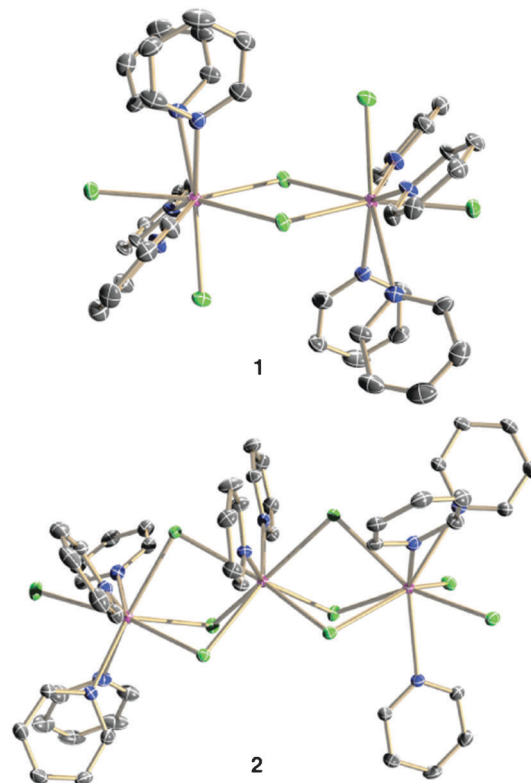
Fig. 2 Molecular structures of 1 (in crystals of 1 · 4\text{C}_5\text{H}_5\text{N} ) and of 2 . Thermal ellipsoids set at 50% probability. Hydrogen atoms and co-crystallized solvent are removed for clarity; U: pink, Cl: green, N: blue, C: dark-grey.
