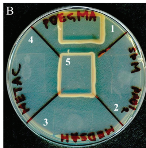
Fig. 5 Motility of P. aeruginosa PAO1 associated with polymer surfaces; a drop of bacterial culture was applied onto an agar plate, dried and covered with a polymer-coated glass slip. Untreated glass was used as a control. Panel A shows the diameter of the ring of bacteria spreading under the coated glass slip after 18 h. Panel B shows a similar experiment after two days. In the case of untreated glass, POEGMA and PMMA, the bacteria placed in the center of the surface reached the edge of the glass slip and started growing around it. In the case of SPM, METAC and MEDSAH, the bacteria only spread in a small circle under the surface. 1 – POEGMA, 2 – SPM, 3 – MEDSAH, 4 – METAC, and 5 – untreated glass.
