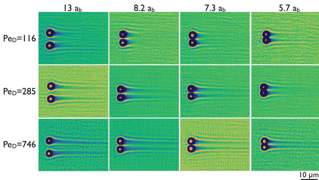
Fig. 2 Microstructure of the bath suspension is organized into two dimensional representations of the time-averaged bath particle density for four probe particle separations and three velocities. The columns represent the probe separations given in terms of the bath particle hydrodynamic radius. The rows are the Péclet numbers defined by eqn (1). Dark colors indicate regions depleted of bath particles, while bright regions have an excess above the average bath suspension density. The bright dot at the center of each depleted region is the position of the probe particle.
