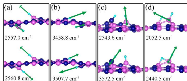
Figure 6 Notable displacement patterns of two hydrogen atoms adsorbed on dh -BN with a) V_N , b) V_B , c) SW, and d) B_N defect. The magenta, blue, black and light blue balls represent the B, N, and H atoms, respectively. Arrows indicate displacement directions.
