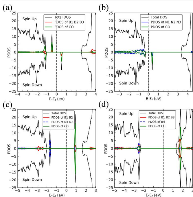
Figure 8 Spin-polarized TDOS (black line), PDOS of defect area (red or blue) and PDOS of adsorbed CO (green line) of CO- dh -BN with (a) V_N , (b) V_B , (c) SW, and (d) B_N , respectively. The position of the Fermi level ( E_F ) is indicated by dashed line.
