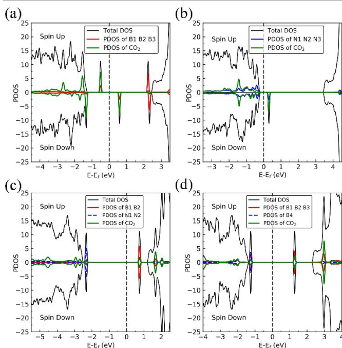
Figure 14 Spin-polarized total density of states (TDOS) (black line), and spin-polarized PDOS of defect area (red line or blue line) and of adsorbed CO 2 (green line) of CO 2 - dh -BN with (a) V N , (b) V B , (c) SW, and (d) B N , respectively. The position of the Fermi level ( E_F ) is indicated by dashed line.
