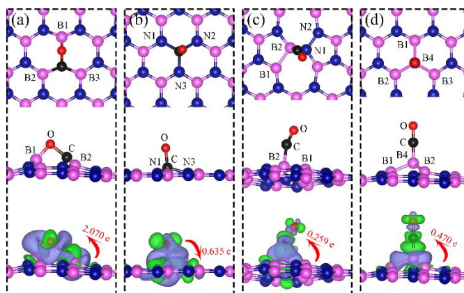
Figure 7 Top and side views of the most energetically favorable configurations of adsorbed CO on dh -BN with a) V_N , b) V_B , c) SW, and d) B_N type defect. The magenta, blue, black and red balls represent the B, N, C, and O atoms, respectively. The top and middle panel shows the top and side views, respectively. Bottom: the corresponding side views of the geometric structures with the charge density difference. The green and violet isosurfaces with iso-value of \pm 0.003 e/ \text{\AA}^3 , represent the accumulation and depletion of electron, respectively. The red arrow shows the electron transfer in direction and value using Bader charge analysis.
