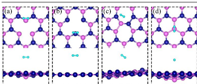
Figure 3 Optimized structures of H_2 adsorbed at favored sites of h -BN with a) V_N , b) V_B , c) SW, and d) B_N . The magenta, blue, white balls represent the B, N and H atoms, respectively. The top and bottom panel shows the top and side views, respectively.
