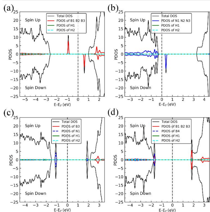
Figure 5 Spin-polarized total density of states (TDOS) (black line), projected density of states (PDOS) in defect regions (red or blue) and spin-polarized PDOS of adsorbed hydrogens (green and cyan) on 2H- dh -BN with (a) V_N , (b) V_B , (c) SW, and (d) B_N , respectively. The position of the Fermi level ( E_F ) is indicated by dashed line.
