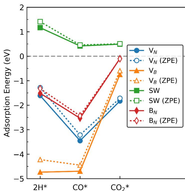
Figure 19 Adsorption energy of 2H, CO, and CO 2 on the dh -BN with (a) V_N , (b) V_B , (c) SW , and (d) B_N , shown with circle, triangle, square, and diamond markers, respectively. Values without and with ZPE corrections are shown in solid and empty markers, respectively. The markers for each defect types are connected with solid or dotted lines for guiding the eyes.
