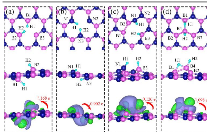
Figure 4 Optimized structures of two hydrogen atoms adsorbed at energetically favorable sites on dh -BN with a) V_N , b) V_B , c) SW, and d) B_N . The magenta, blue, cyan balls represent B, N and H atoms, respectively. The top and middle panel show the top and side views, respectively. Bottom panel: corresponding side view of geometric structure with charge density difference plot. The green and violet isosurfaces with isovalue of \pm 0.003 \text{ e}/\text{\AA}^3 , represent accumulation and depletion of charge, respectively. The red arrow shows the direction of electron transfer evaluated with Bader charge analysis.
