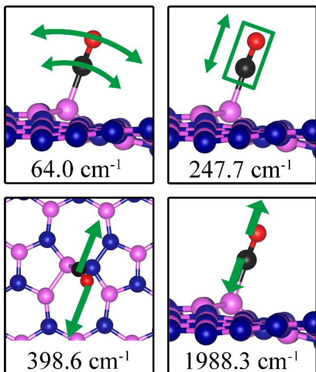
Figure 11 Notable vibrational modes of CO adsorption on dh -BN with SW defect. The magenta, blue, black and red balls represent the B, N, C, and O atoms, respectively. Arrows indicate vibrational patterns. The rectangular encloses the atoms that concertedly move.
