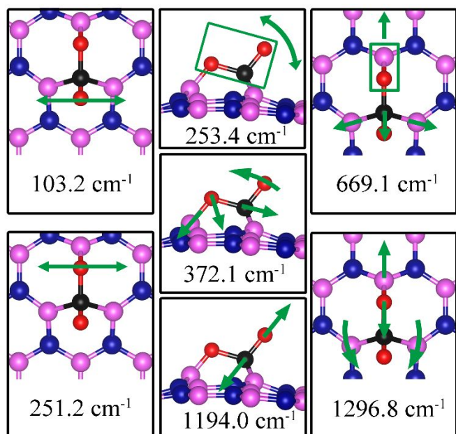
Figure 15 Notable vibrational modes of CO 2 adsorption on dh -BN with V N . The magenta, blue, black and red balls represent the B, N, C, and O atoms, respectively. Arrows indicate vibrational patterns. The rectangular encloses the atoms that move together.
