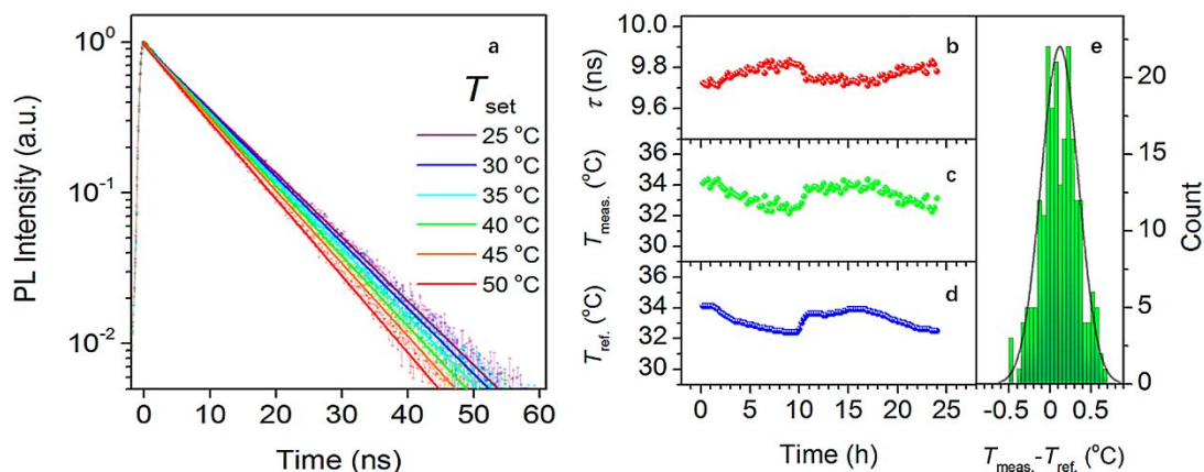
Figure 9. (a) PL emission decays of HeLa cells cultured in CDs aqueous solution with a concentration of 500 \mu\text{g/mL} at different temperatures; (b) PL decay lifetimes extracted from the PL transients recorded every 15 min for 24 h of HeLa cells cultured in CDs aqueous solution (500 \mu\text{g/mL} ); (c) Temperatures obtained using the calibration curve based on a calibration curve described by an equation: T = 330.59 - 94.99\tau + 11.87\tau^2 - 0.54\tau^3 , R_{\text{adj}}^2 = 0.998 , T , temperature; \tau , lifetime; (d) Temperatures measured by a reference thermometer; (e) Histogram revealing the deviation between (c) and (d), the solid line is the distribution curve. Figure adapted from Ref. 23 with permissions from the American Chemical Society.
