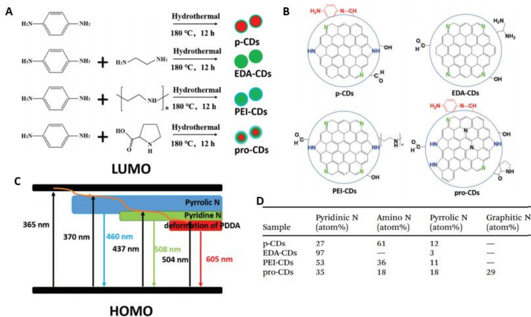
Figure 11: (A) Summary of preparation of CDs. (B) Proposed representative structure for each CDs. (C) Proposed energy level diagram for surface states of CDs. (D) Nitrogen percentages in CDs samples. Figures adapted from Ref. 127 with permissions from The Royal Society of Chemistry.
