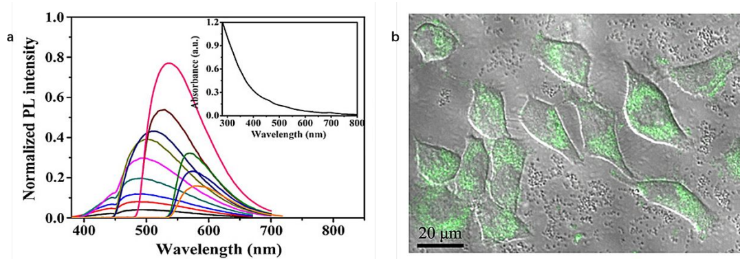
Figure 5. (a) Normalized PL emission spectrum with excitation wavelength increasing from 310 nm in 20 nm increment (inset: UV/vis absorption spectrum of CDs obtained); (b) Confocal microscopy image of Hela cell incubated with CDs ( \lambda_{\text{exc}} = 488 nm). Figure adapted from Ref. 82 with permissions from Elsevier.
