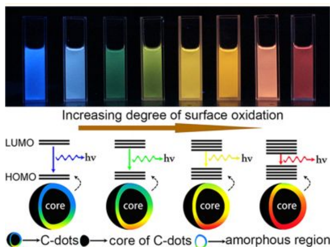
Figure 10: Image of different CDs fractions under UV light and the modeling of their bandgap based on surface oxidation. Figure adapted from Ref. 122 with permissions from the American Chemical Society.
