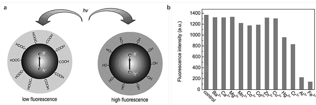
Figure 6. (a) The schematic illustration of PL emission of hydroxyls-coated CDs better than the regular carboxyls-coated CDs ( e^- : electrons, h^+ : holes); (b) The PL quenching effect of CDs by different metal ions ( \lambda_{exc} = 310 nm). Figure adapted from Ref. 20 with permissions from Springer.
