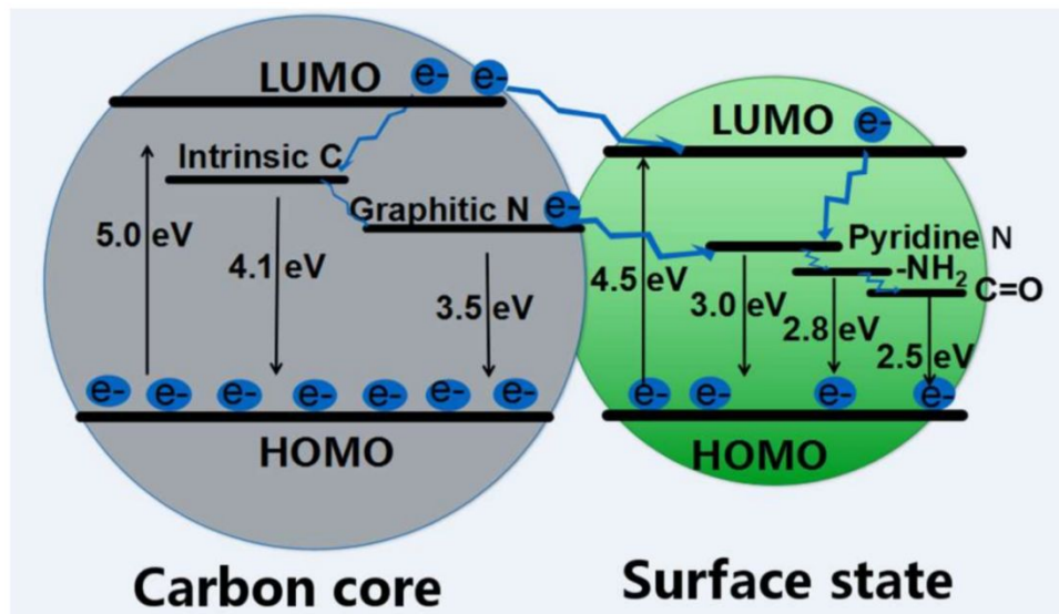
Figure 12: A scheme of energy band structure and possible PL process for CDs. Figure adapted from Ref. 163 with permission from MDPI.
