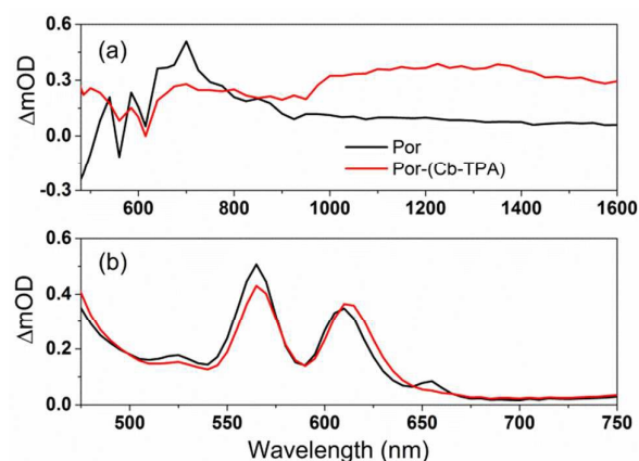
Figure 5. (a) Transient absorption spectra of \text{TiO}_2 -Por and \text{TiO}_2 -Por-(Cb-TPA) in the presence of the inert electrolyte \text{I}_0 at 10 \mu\text{s} time delay following laser excitation (532 nm, 24~26 \mu\text{J cm}^{-2} pulse ^{-1} ) and (b) absorbance of \text{TiO}_2 -Por and \text{TiO}_2 -Por-(Cb-TPA).
