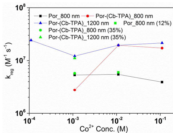
Figure 9. Regeneration rate constant of Por and Por-(Cb-TPA) versus the concentration of Co^{2+} . Por with 12% dye-loading probed at 800 nm and Por-(Cb-TPA) with 35% dye-loading probed at 800 nm and 1200 nm are also shown.
