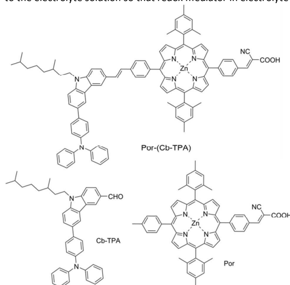
Figure 2. Chemical structures of the compounds
