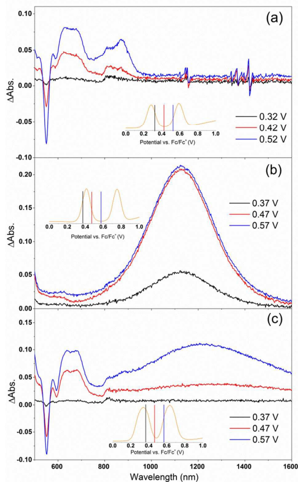
Figure 4. Spectro-electrochemical (SEC) spectra of (a) Por, (b) Cb and (c) \text{Por}-(\text{Cb-TPA}) at different oxidation potentials vs. \text{Fc}/\text{Fc}^+ . For wavelength range from 230 nm, see Fig. S4.
