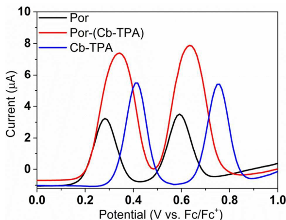
Figure 3. (a) Differential pulse voltammetry of the compounds measured in dichloromethane solutions
