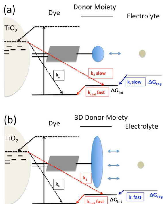
Figure 1. Utilization of intramolecular hole transfer to enhance dye cation regeneration. (a) reduced recombination and slower regeneration kinetics; (b) faster dye regeneration kinetics at a smaller driving force using a tridimensional donor moiety.
