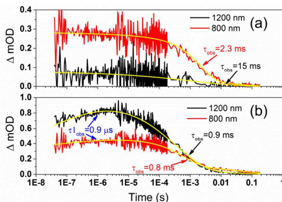
Figure 6. Transient absorption decays and fitted functions of (a) \text{TiO}_2 -Por and (b) \text{TiO}_2 -Por-(Cb-TPA) with the inert electrolyte \text{I}_0 (532 nm, 45-50 \mu\text{J cm}^{-2} pulse ^{-1} ; repetition rate 1 Hz).
