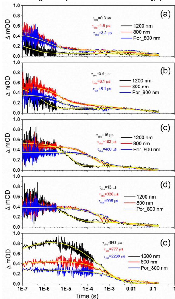
Figure 7. Transient absorption decay and fitted curves of \text{TiO}_2\text{-Por-(Cb-TPA)} probed at 1200 nm (black) and 800 nm (red) and \text{TiO}_2\text{-Por} probed at 800 nm (blue) with five \text{I}^-/\text{I}_3^- electrolytes after pulsed 532 nm laser irradiation. (a) \text{I}^-_1 , (b) \text{I}^-_{0.1} , (c) \text{I}^-_{0.01} , (d) \text{I}^-_{0.001} and (e) \text{I}^-_0 (532 nm, 45\text{-}50\mu\text{J cm}^{-2}\text{ pulse}^{-1} ; repetition rate 1 Hz).
