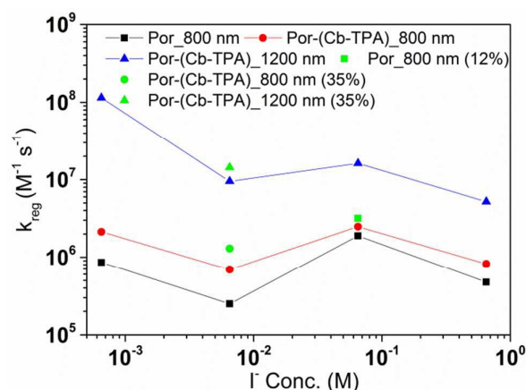
Figure 8. Regeneration rate constant of Por and Por-(Cb-TPA) versus the concentration of I^- . Por with 12% dye-loading probed at 800 nm and Por-(Cb-TPA) with 35% dye-loading probed at 800 nm and 1200 nm are also shown.
