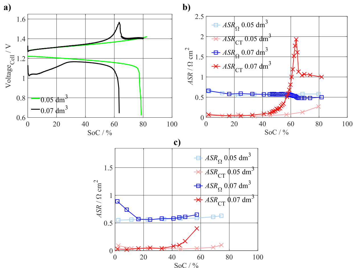
Figure 4: a) U - Q_{\text{areal}} dependence of a charge-discharge cycle for two different negolyte volumes with the same 80% SoC charging limit; ASR_{CT} and ASR_{\Omega} evaluated from GEIS_{LOAD} measured during the battery for b) charging and c) discharging phase of the initial cycle. Experimental conditions: Std. electrolyte composition, Current density: 100 mA cm -2 ; Operating temperature: 40 °C; Electrolyte flow rate: 0.08 dm 3 min -1 .
