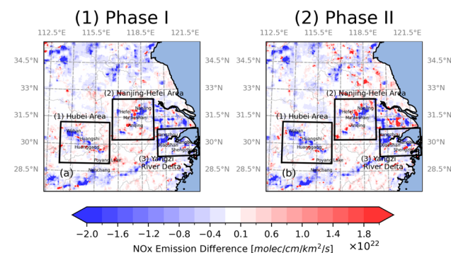
Fig. 2 Spatial distribution of NO x emission differences between lockdown phases and pre-lockdown baseline over eastern China. (a) Phase I (strict lockdown) and (b) Phase II (early recovery) emission changes. Black boxes denote three study regions: (1) Region I: Hubei Area, (2) Region II: Nanjing–Hefei Area, and (3) Region III: Yangtze River Delta. Negative values (blue) indicate emission reductions; positive values (red) indicate increases.
