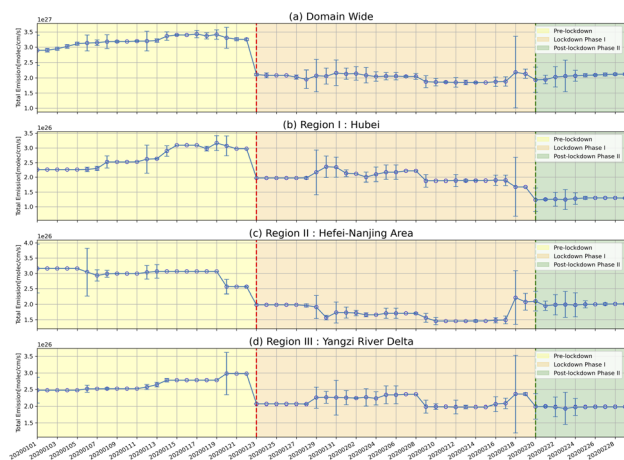
Fig. 1 Temporal evolution of NO x emissions during the COVID-19 outbreaks. Daily NO x emissions from January to March 2020 for (a) all domains, (b) Region I: Hubei Province, (c) Region II: Hefei–Nanjing Area, and (d) Region III: Yangtze River Delta. Background shading indicates pre-lockdown (yellow), Phase I lockdown (orange), and Phase II recovery (green) periods. Red and green vertical lines mark lockdown initiation (23 January) and relaxation (20 February), respectively. Error bars show daily inversion uncertainties.
