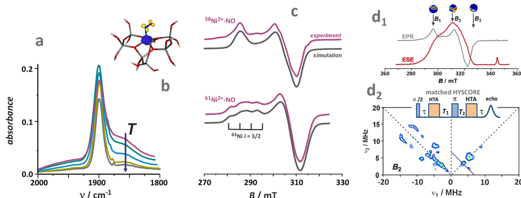
Fig. 33 Spectroscopic evidence of the formation of nitrosyl upon NO interaction with \text{Ni}^{2+} /ZSM-5. The IR spectra of NO adsorption at various temperatures (a), spin density contour of the [\text{NiNO}]^{2+} adduct in ZSM-5 (b), CW-EPR spectra (77 K) of NO adsorption on Ni and isotopically enriched ^{61}\text{Ni} ( I = 3/2 ) hosted in ZSM-5 zeolite (c), electron spin echo detected EPR signal (10 K), the arrows indicate observer positions ( B_1 , B_2 , B_3 ) at which HYSCORE signals can be measured ( d_1 ). HYSCORE spectrum due to the ^{14}\text{N} hyperfine interaction recorded at B_2 position with the matched pulse sequence ( d_2 ). The figure was based on data from ref. 156 and 247.
