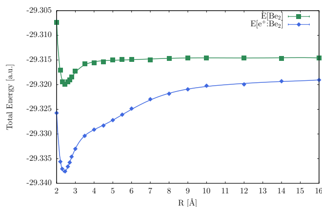
Fig. 1 Potential energy curve for Be 2 (green) and e + :Be 2 (blue) computed at the DMC level. Error bars represent one standard error on the mean.
