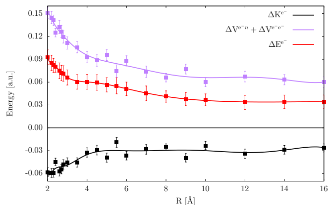
Fig. 4 Deformation energy contributions, differences between E^{\text{e}^+}[\text{e}^+:\text{Be}_2] - E^{\text{e}^+}[\text{Be}_2] electronic energy components. Error bars represent one standard error on the mean.
