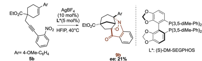
Scheme 8 Formation of 9 via a [2 + 2 + 1] cycloaddition.
