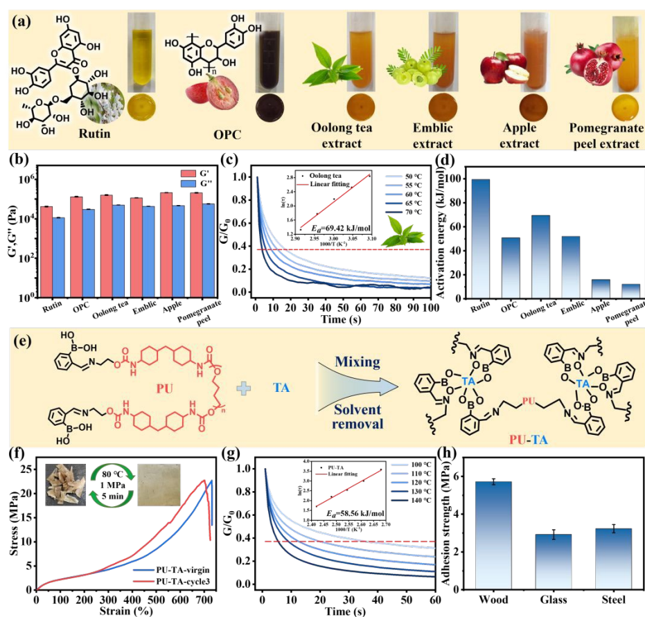
Fig. 5 Preparation of various vitrimers. (a) Structure diagram of natural polyphenols, the inserts are optical photo of three-component mixture and dried films from different polyphenols. (b) The storage modulus ( G' ) and the loss modulus ( G'' ) of different vitrimers. These studies were carried out conducted at 0.1% strain and an angular frequency of 1 Hz. (c) Stress relaxation plots of vitrimers from Oolong tea extract. (d) Activation energy of vitrimers from various polyphenols. (e) Synthesis route of PU-TA. (f) Stress-strain curves, (g) stress relaxation plots and (h) adhesion strength of PU-TA.
