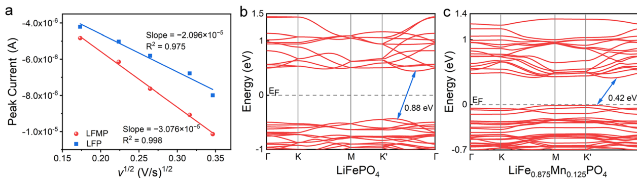
Fig. 2 (a) Plots of the current of the reduction peak ( I_p ) of LFMP and LFP versus the square root of the electrode scanning rate ( v^{1/2} ). Energy band diagrams of LFP (b) and \text{LiFe}_{0.875}\text{Mn}_{0.125}\text{PO}_4 (c).
