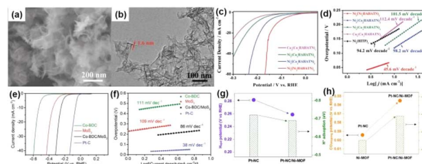
Fig. 6 (a) SEM image and (b) TEM image of \text{Ni}_3(\text{Ni}_3\text{·HAHATN})_2 nanosheets. (c) LSV plots of \text{M}_2\text{M}_3(\text{M}_1\text{·HAHATN})_2 and (d) Tafel plots. 89 (e) The polarization curves of MoS 2 , Co-BDC and Co-BDC/MoS 2 and so on. (f) Tafel plots of catalysts. 90 (g) Graphs showing the Hupd desorption peak potentials derived from cyclic voltammetry (CV) plots, as well as the H* adsorption energy predicted through density functional theory (DFT) calculation. (h) Graph of CO stripping peak potentials. 91
