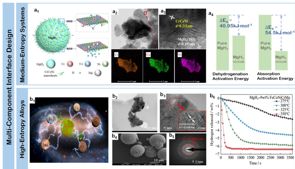
Fig. 8 (a1) Mechanism diagram of dehydrogenation and rehydrogenation of the CrCoNi catalyzed \text{MgH}_2/\text{Mg} system; (a2 and a3) HRTEM image and elemental mapping of \text{MgH}_2 + 9 \text{ wt\% CrCoNi} ; (a4) energy diagram for hydrogen absorption and desorption of \text{MgH}_2 + 9 \text{ wt\% CrCoNi} . 119 (b1) Mechanism diagram of dehydrogenation (DEH) and rehydrogenation (REH) of the FeCoNiCrMo catalyzed \text{MgH}_2/\text{Mg} system; (b2) TEM and (b3) HRTEM of ball-milled FeCoNiCrMo; (b4) SEM of as-received FeCoNiCrMo; (b5) SAED of ball-milled FeCoNiCrMo; (b6) \text{MgH}_2-9 \text{ wt\% FeCoNiCrMo} in isothermal mode. 120
