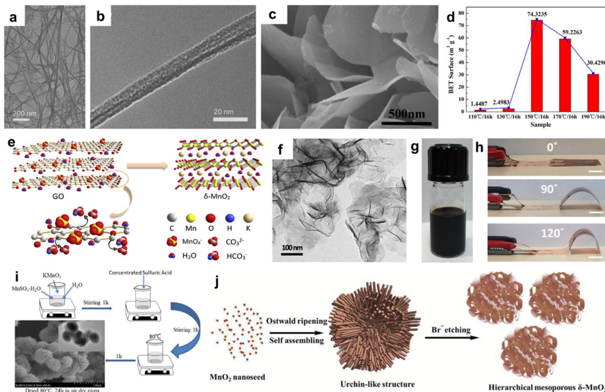
Fig. 6 (a and b) TEM images of KMO NNT. 69 Reproduced with permission from ref. 69. Copyright 2021, Elsevier. (c) SEM image of \delta\text{-MnO}_2 at 150 °C, (d) Specific surface area of \delta\text{-MnO}_2 at various temperatures. 87 Reproduced with permission from ref. 87. Copyright 2016, Elsevier. (e) Illustration of the formation of \delta\text{-MnO}_2 nanosheets. (f) TEM image of the as-prepared \delta\text{-MnO}_2 nanosheets. 88 Reproduced with permission from ref. 88. Copyright 2019, Elsevier. (g) Image of the formulated \delta\text{-MnO}_2 nanosheet ink. (h) Optical images of MSC bent under different angles. 89 Reproduced with permission from ref. 89. Copyright 2018, Elsevier. (i) Schematic for the preparation of spherical \delta\text{-MnO}_2 nanoflowers. 90 Reproduced with permission from ref. 90. Copyright 2024, the American Chemical Society. (j) Plausible mechanism involved in the growth of mesoporous \delta\text{-MnO}_2 nanostructures. 91 Reproduced with permission from ref. 91. Copyright 2016, the Royal Society of Chemistry.
