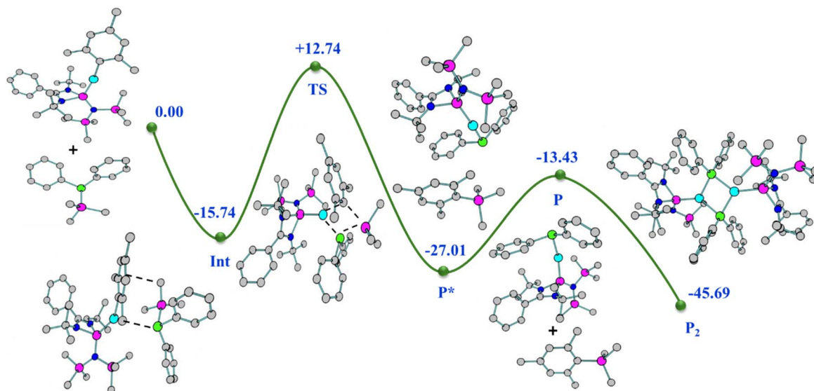
Fig. 11 Relative energy (kcal mol -1 ) (not drawn to scale) reaction profile for the formation of complex 23 from complex 2 with PPh 2 SiMe 3 .
