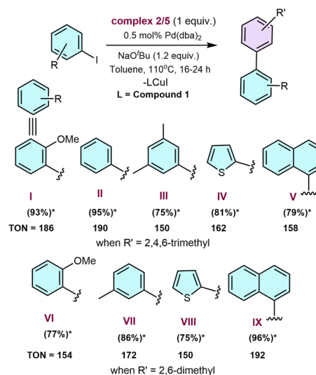
Scheme 7 Pd-catalysed sp 2 –sp 2 C–C coupling reaction using 2 and 5 as an aryl transfer agent. *Isolated yields.
